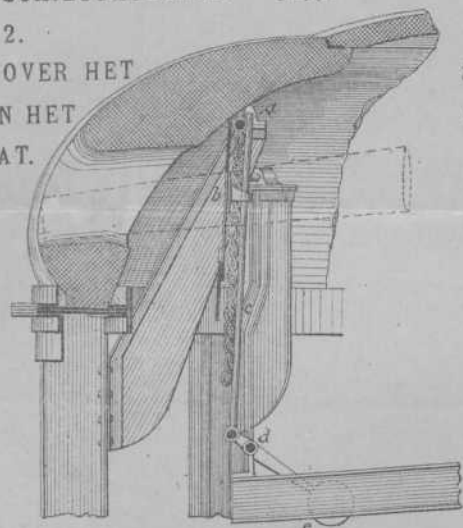
SCHIETGATBLIND. 1:40.
