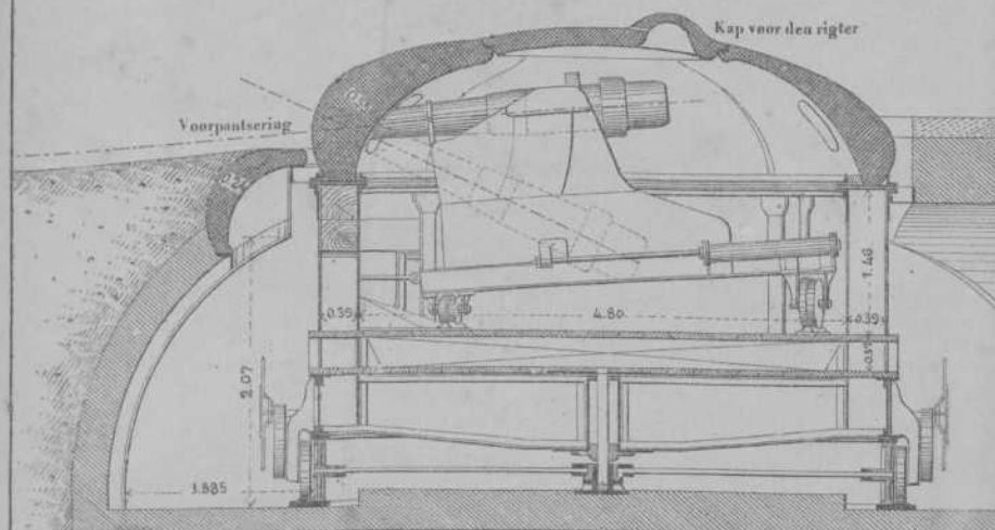
SCHIETGATBLIND. 1:40.
