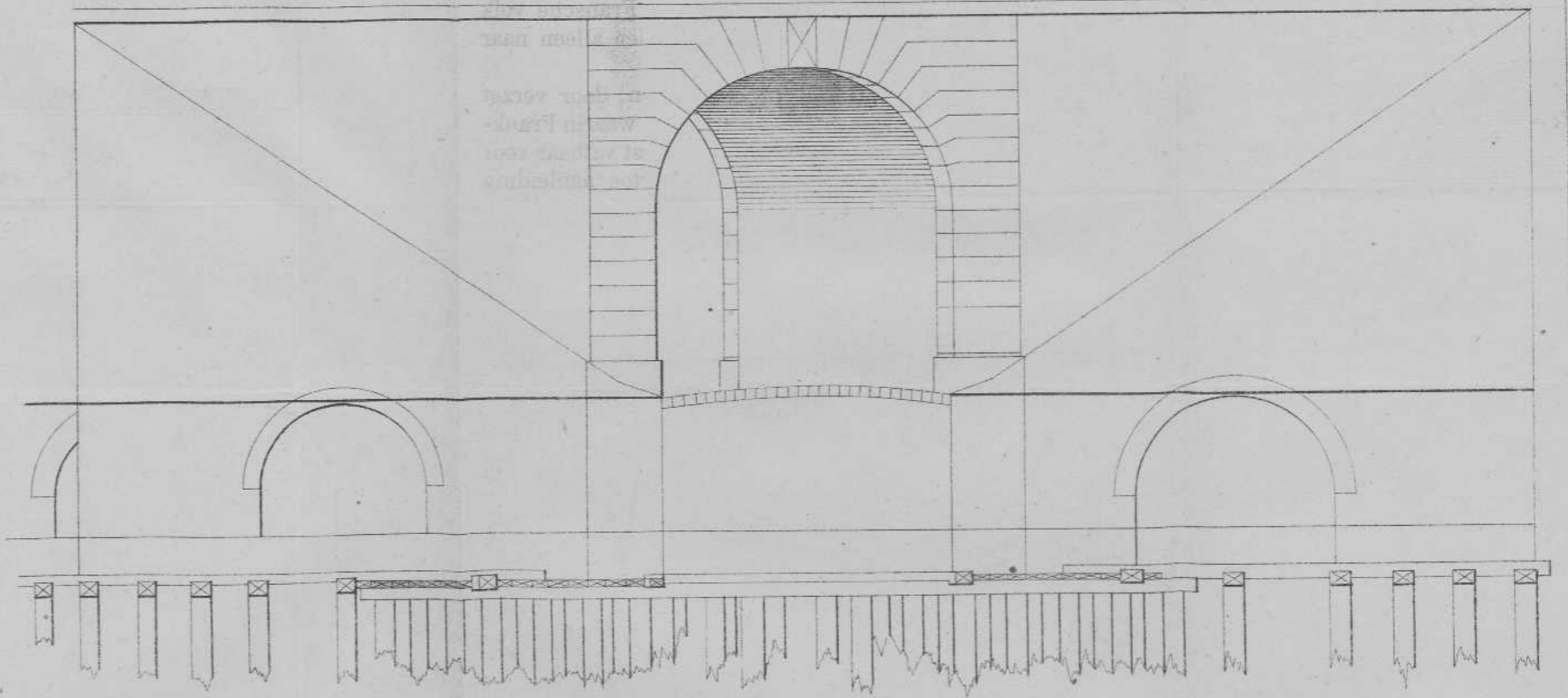
Fig. 2b (1:100)
