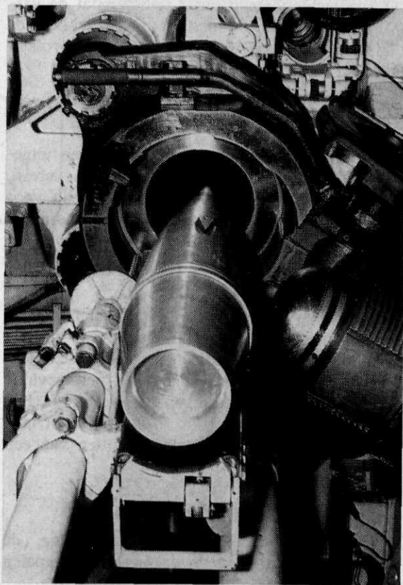
Afb. 10 Prototype in de M109
