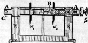
Fig. III.a STEREO-MICROMETER
